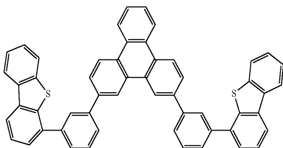
Compound 4'
