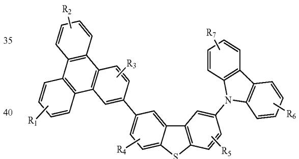
Compound 15'G
