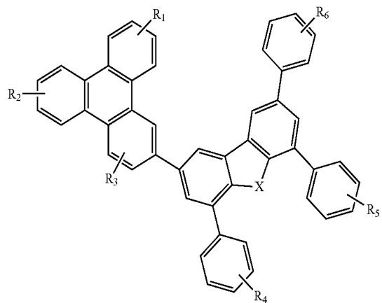
Compound 35 G
