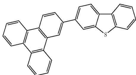
Compound 8'
