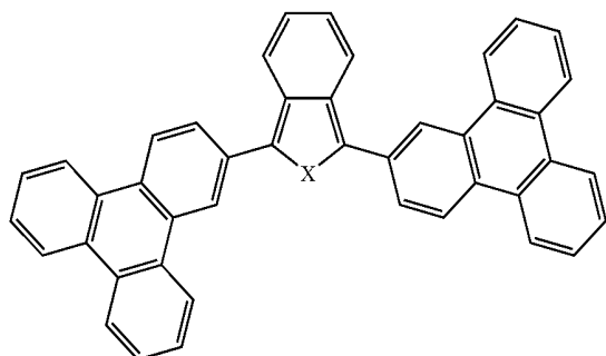
Compound 11
