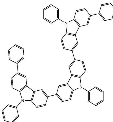
Compound HTL1-4
