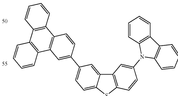
Compound 15'
