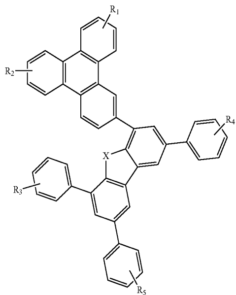
Compound 32 G
