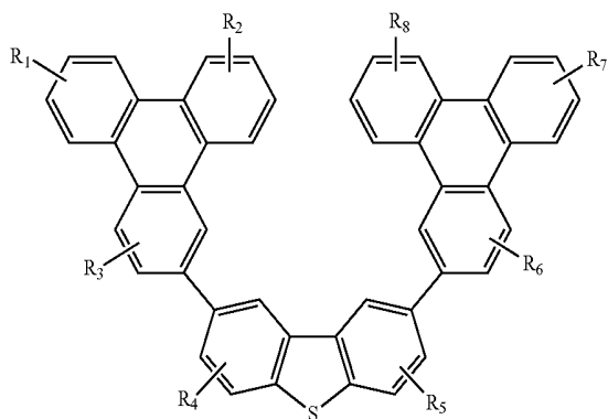
Compound 5'G
