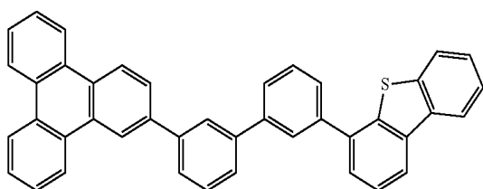
Compound 9'
