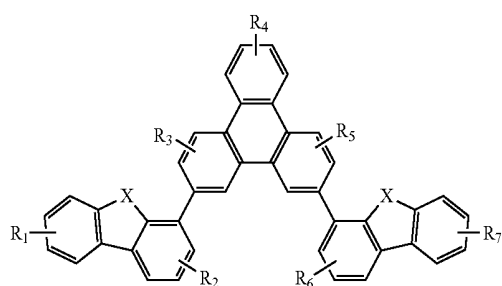
Compound 10G
