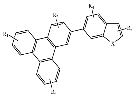
Compound 17
