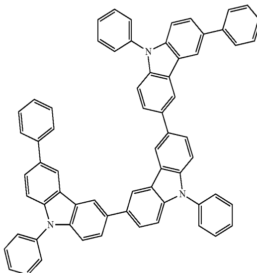
Compound HTL1-2
