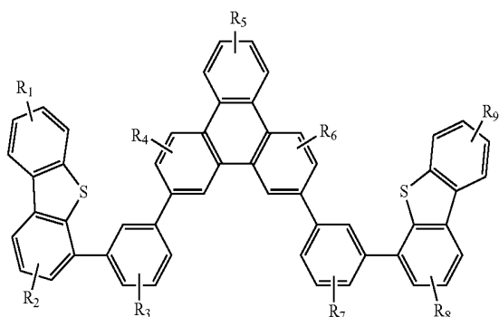
Compound 4'G
