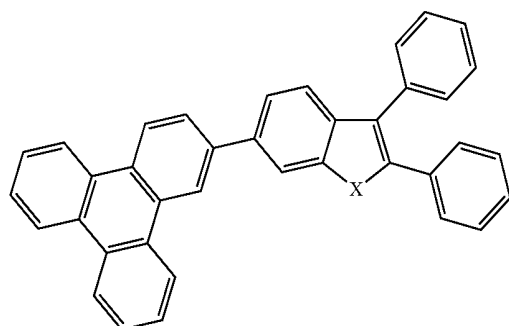
Compound 18G
