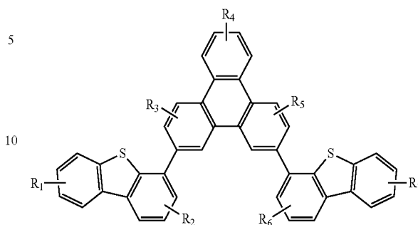
Compound 10'
